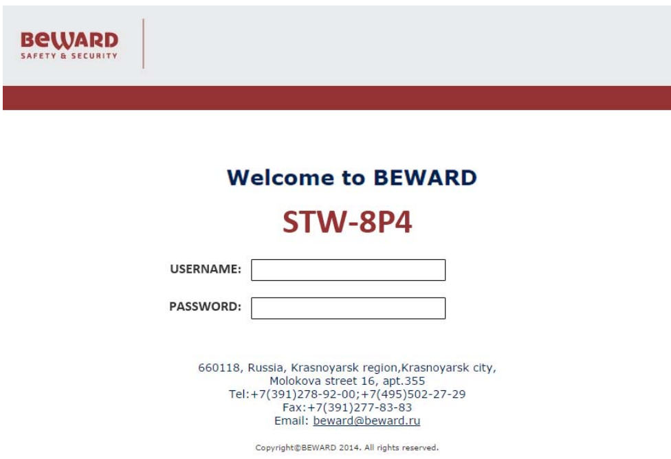
Figure 3-2 Login screen
