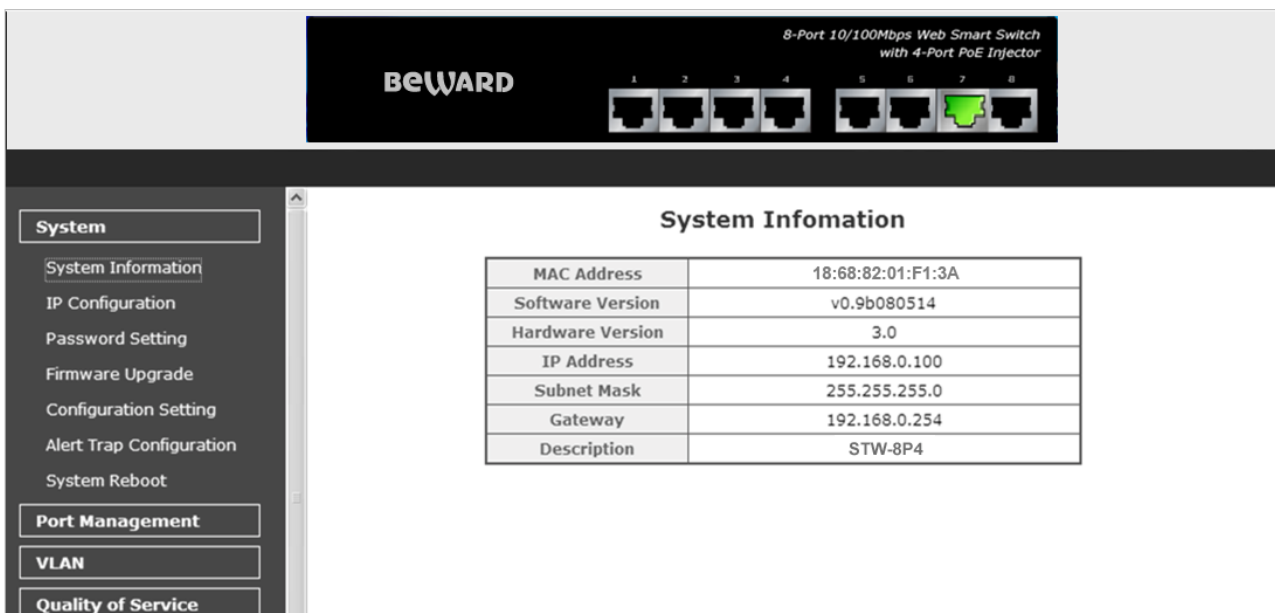
Figure 4-3 System screen
